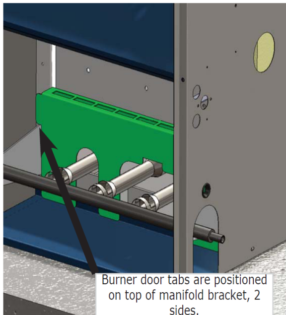
Figure 1 - Replacement Burner Door with Tabs
