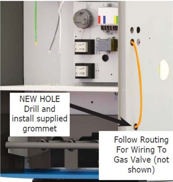
Figure 5 - Gas Valve and Spark Wiring Relocation
