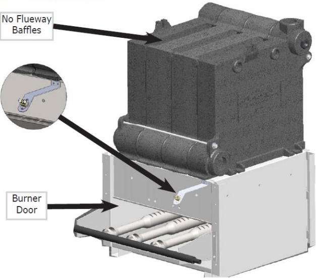
Figure 6 - Replacement Heat Exchanger
